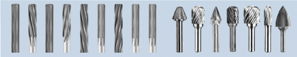
REAMER TOOLS
