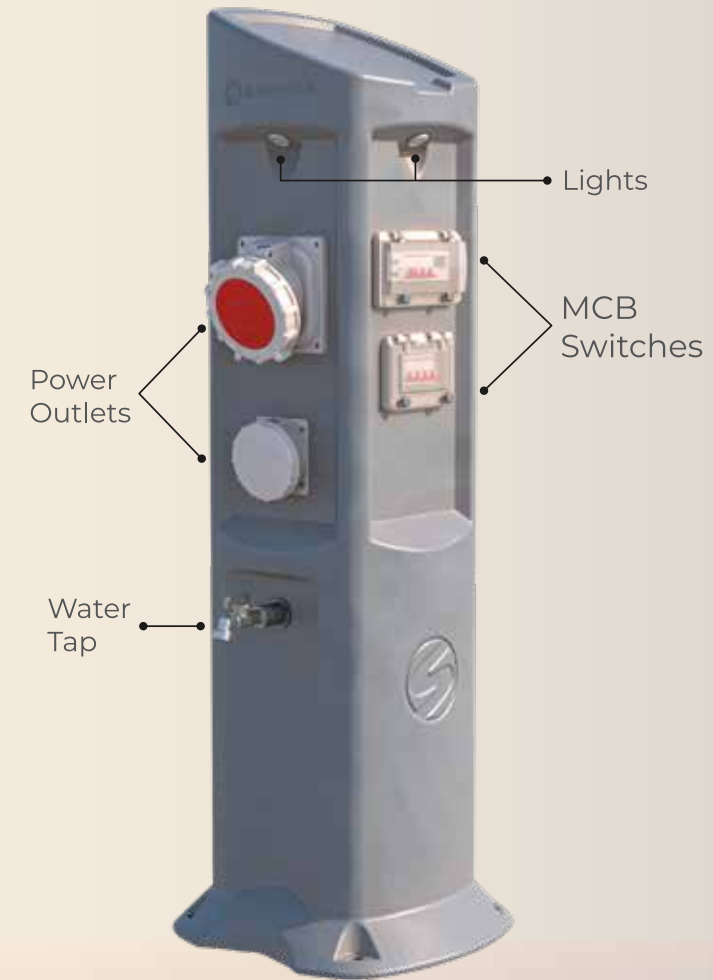
Light/Utility Pedestal
