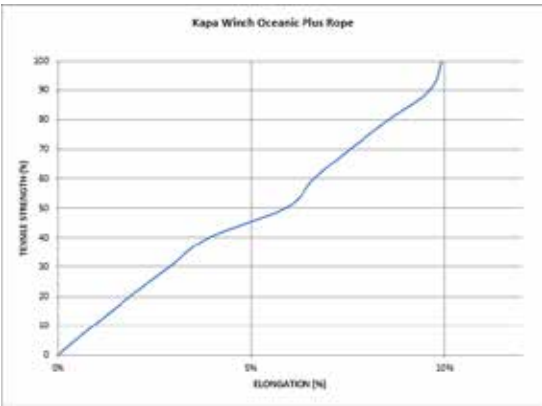
LOAD ELONGATION CURVE
