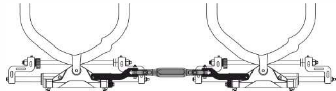
Fig. D : Dual Cylinders - Dual Outboards Heavy Duty Tie Rod
