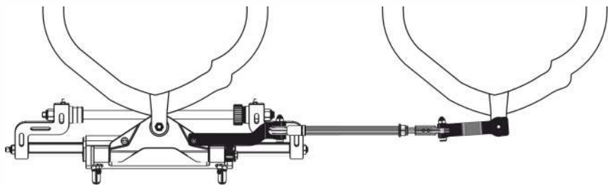
Fig. B : Single Cylinder - Dual Outboards
