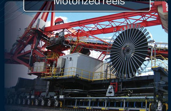
Motorized reels
